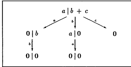
Figure 2-3: Derivation tree for a \mid b + c .
