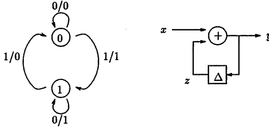
Figure 2-3: Implementation of the Modulo-2 Counter
