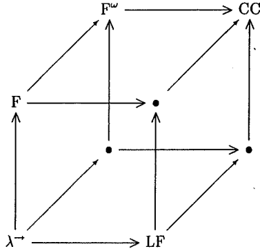
Figure 1-1: Barendregt's cube
